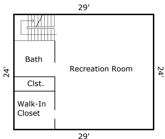
Pool House Second Floor [696 Sq ft]
