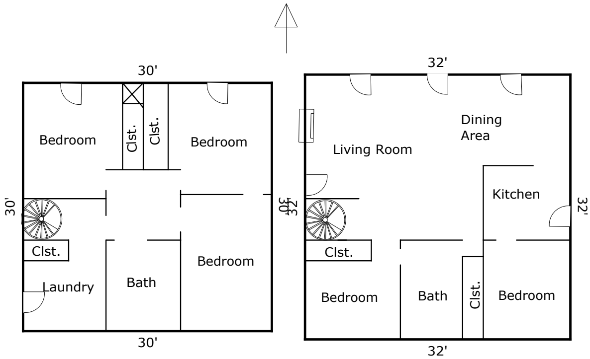
Residence First Floor [900 Sq ft]
